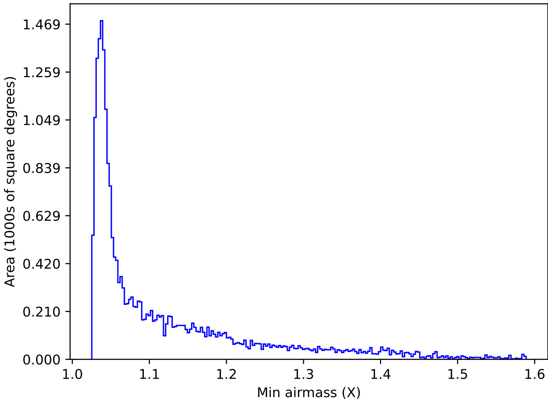
all_long_v3.4_10yrs All sky u band: Min airmass
