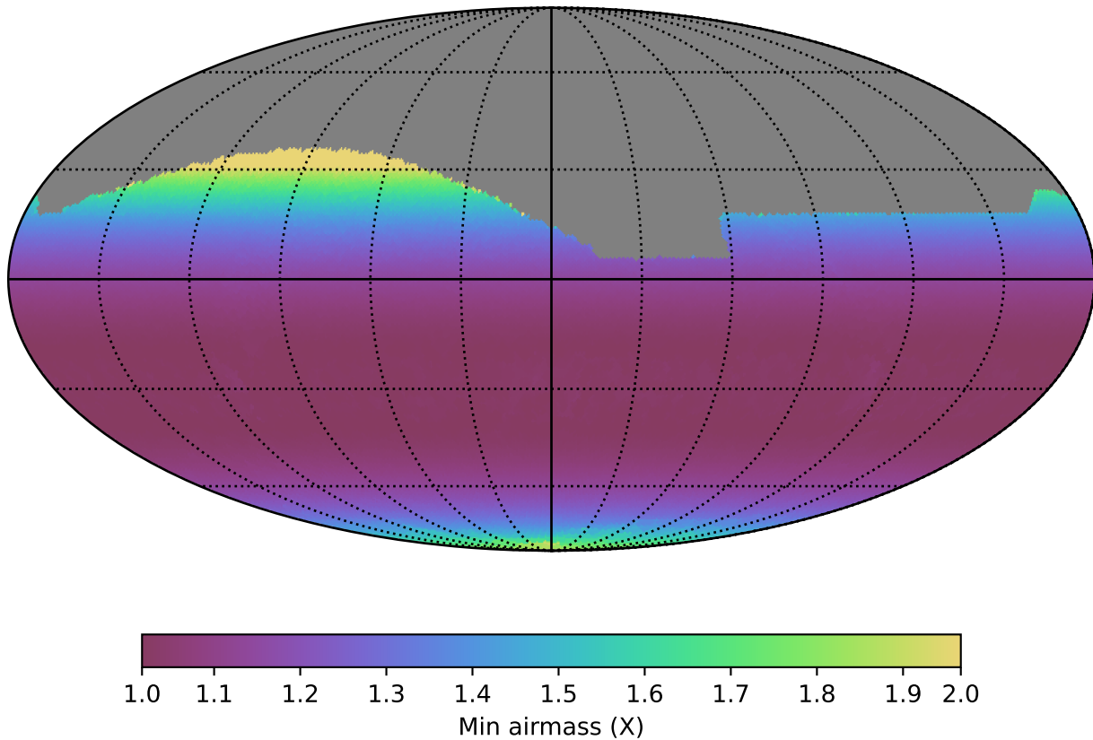
all_long_v3.4_10yrs All sky r band: Min airmass
