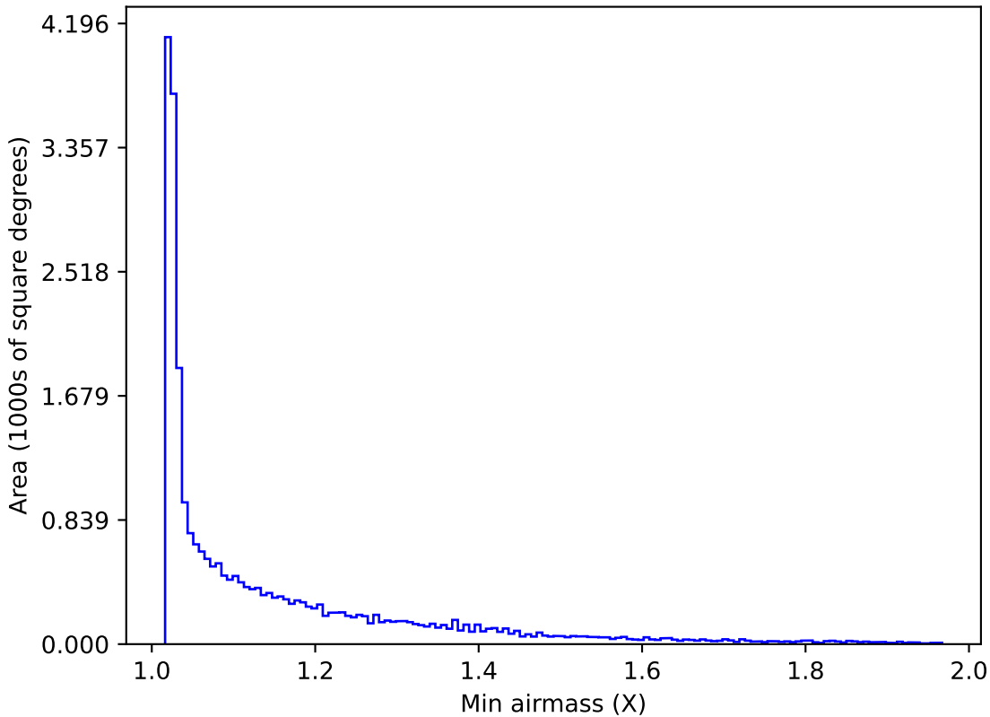
all_long_v3.4_10yrs All sky r band: Min airmass
