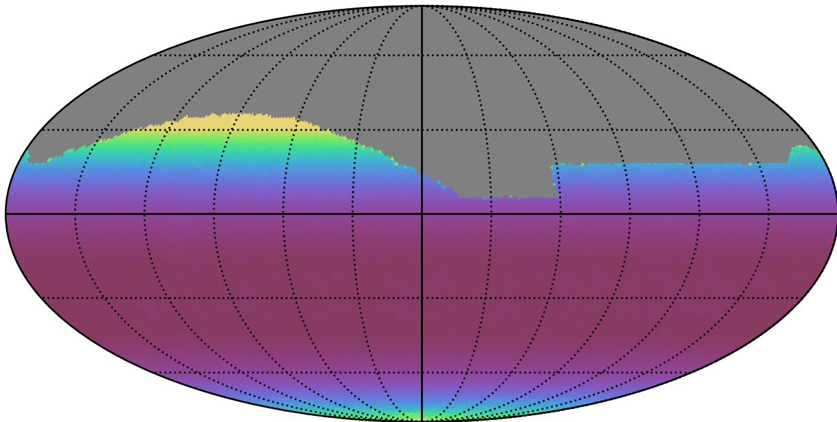
all_long_v3.4_10yrs All sky i band: Min airmass
