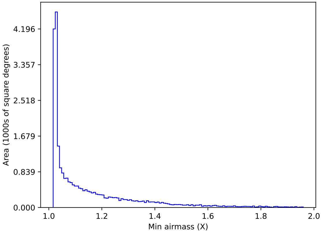
all_long_v3.4_10yrs All sky i band: Min airmass
