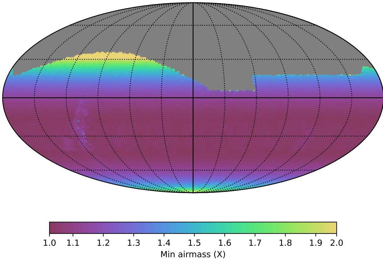
all_long_v3.4_10yrs All sky g band: Min airmass
