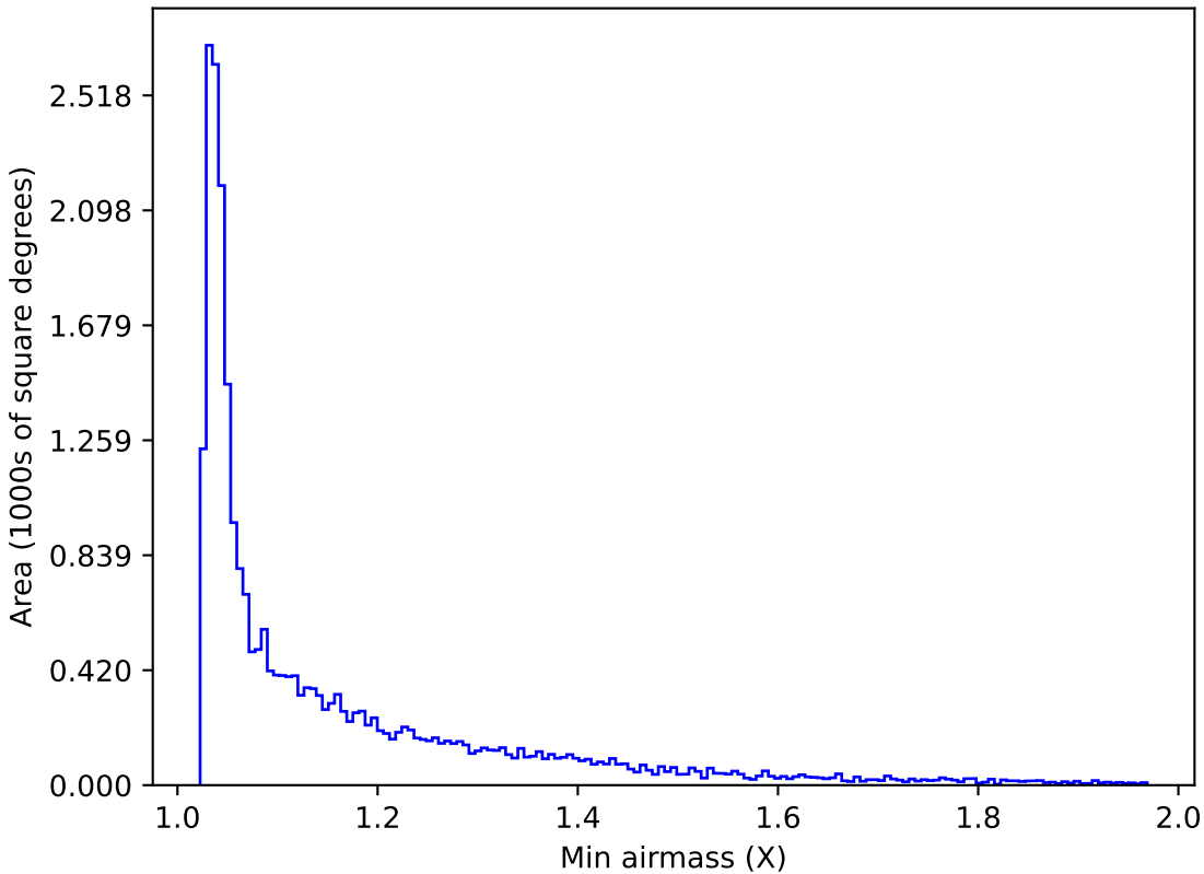
all_long_v3.4_10yrs All sky g band: Min airmass
