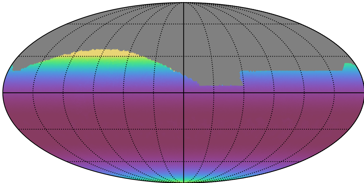
all_long_v3.4_10yrs All sky all bands: Min airmass
