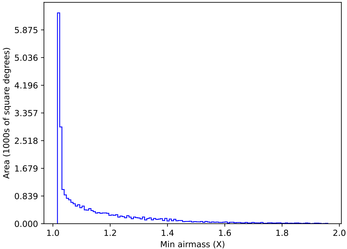
all_long_v3.4_10yrs All sky all bands: Min airmass
