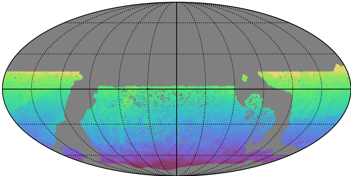
all_long_v3.4_10yrs WFD all bands: Min HA
