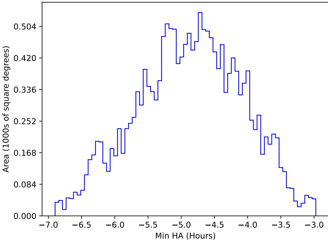
all_long_v3.4_10yrs WFD all bands: Min HA
