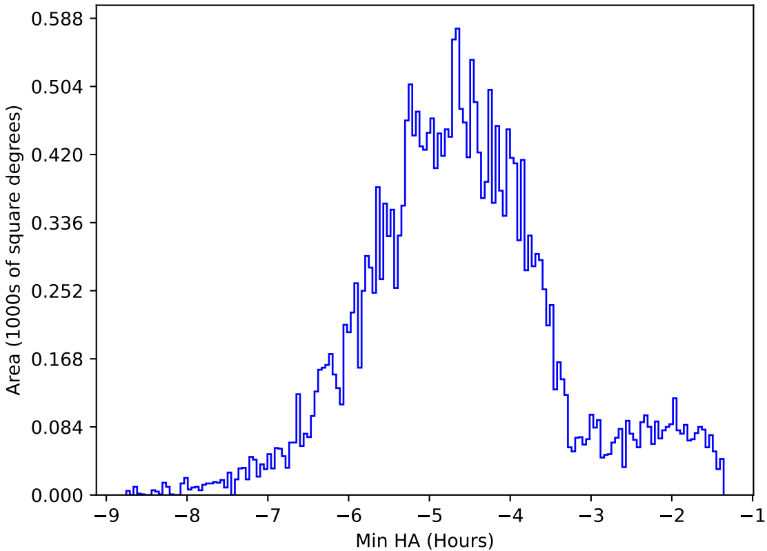
all_long_v3.4_10yrs All sky all bands: Min HA
