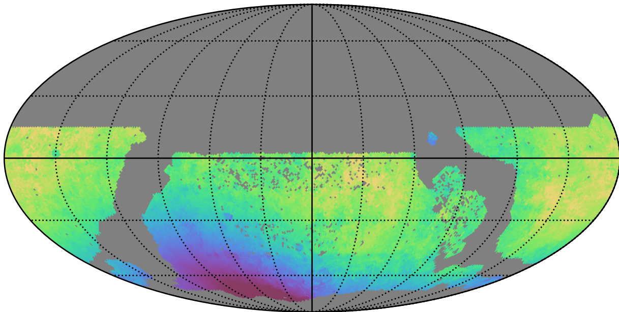
all_long_v3.4_10yrs WFD y band: Median solarElong
