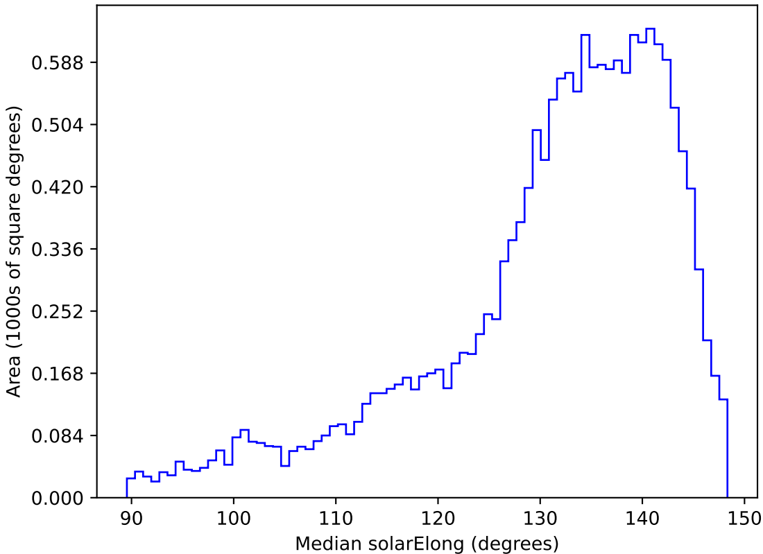
all_long_v3.4_10yrs WFD y band: Median solarElong
