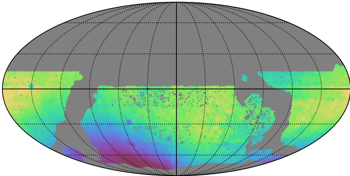
all_long_v3.4_10yrs WFD r band: Median solarElong
