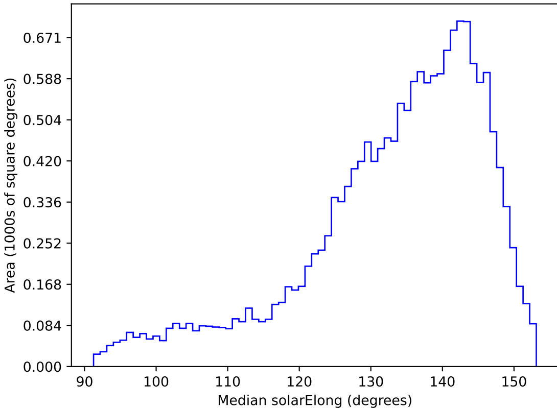
all_long_v3.4_10yrs WFD r band: Median solarElong
