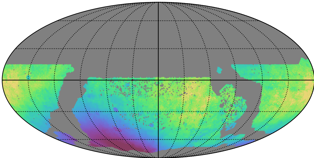
all_long_v3.4_10yrs WFD i band: Median solarElong
