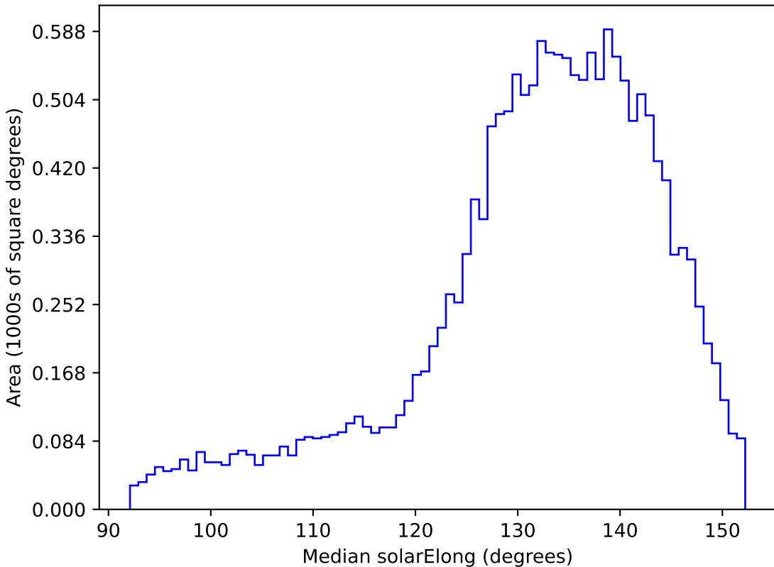
all_long_v3.4_10yrs WFD i band: Median solarElong
