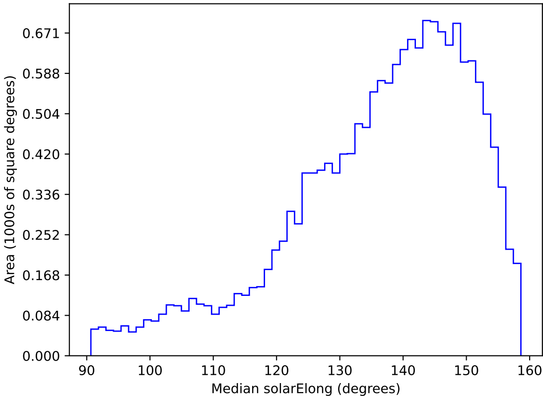
all_long_v3.4_10yrs WFD g band: Median solarElong
