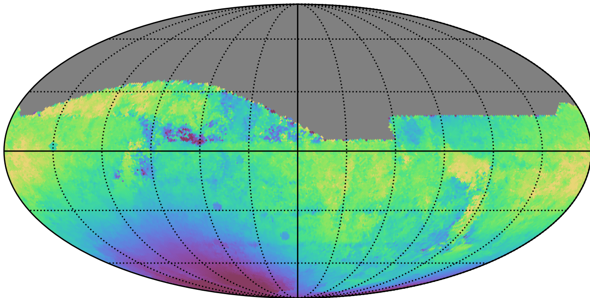
all_long_v3.4_10yrs All sky z band: Median solarElong
