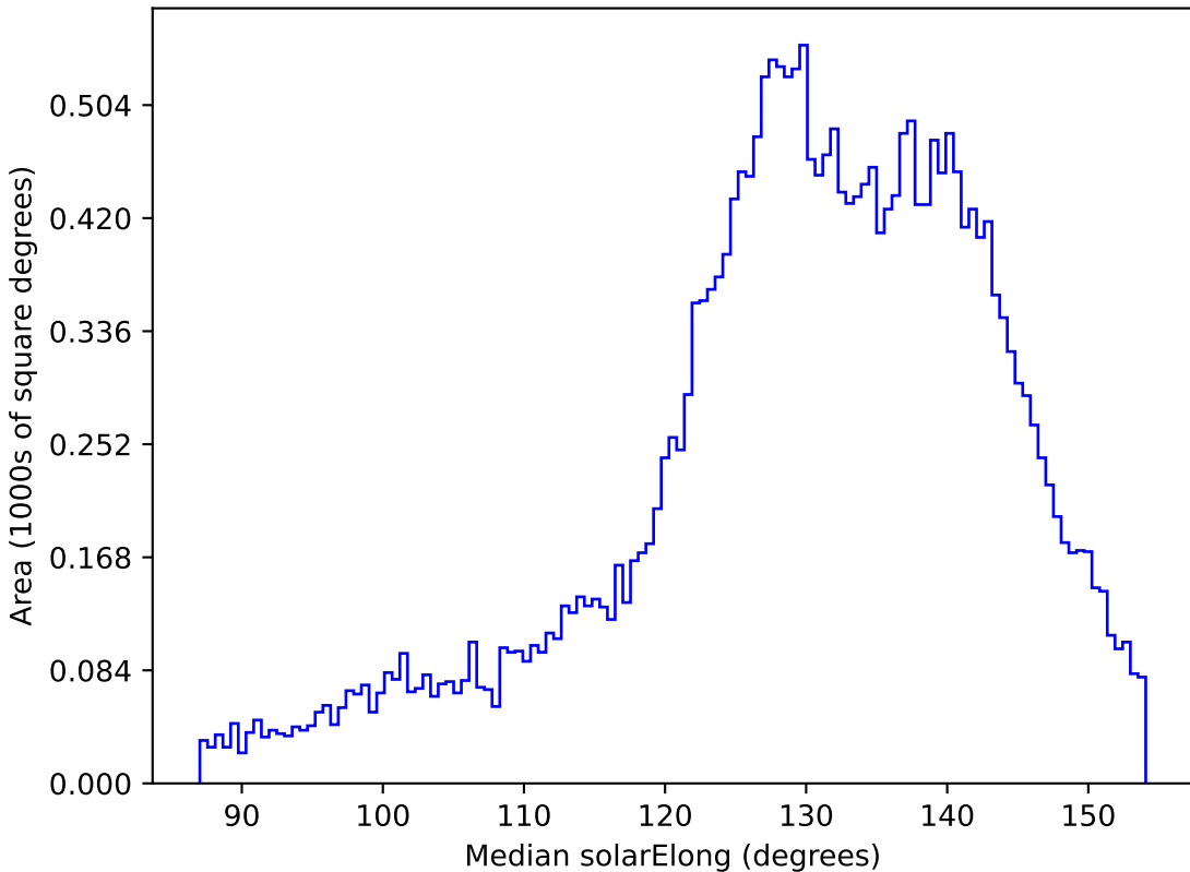
all_long_v3.4_10yrs All sky z band: Median solarElong
