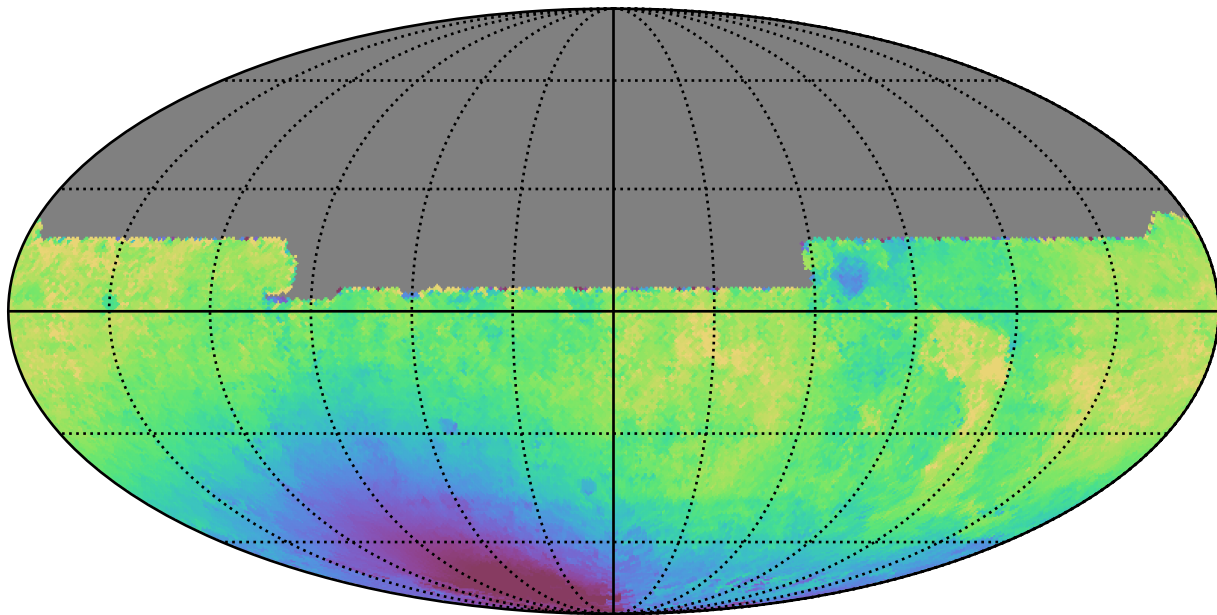
all_long_v3.4_10yrs All sky y band: Median solarElong
