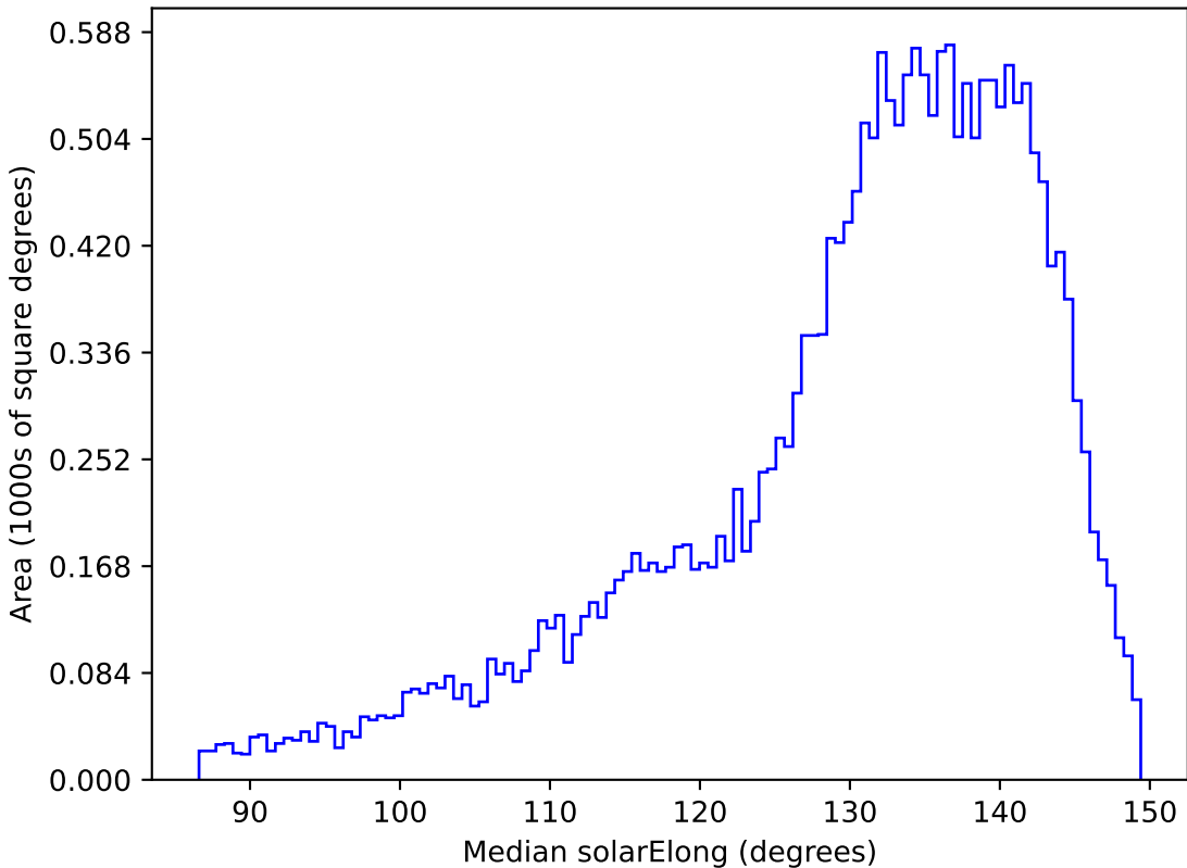
all_long_v3.4_10yrs All sky y band: Median solarElong
