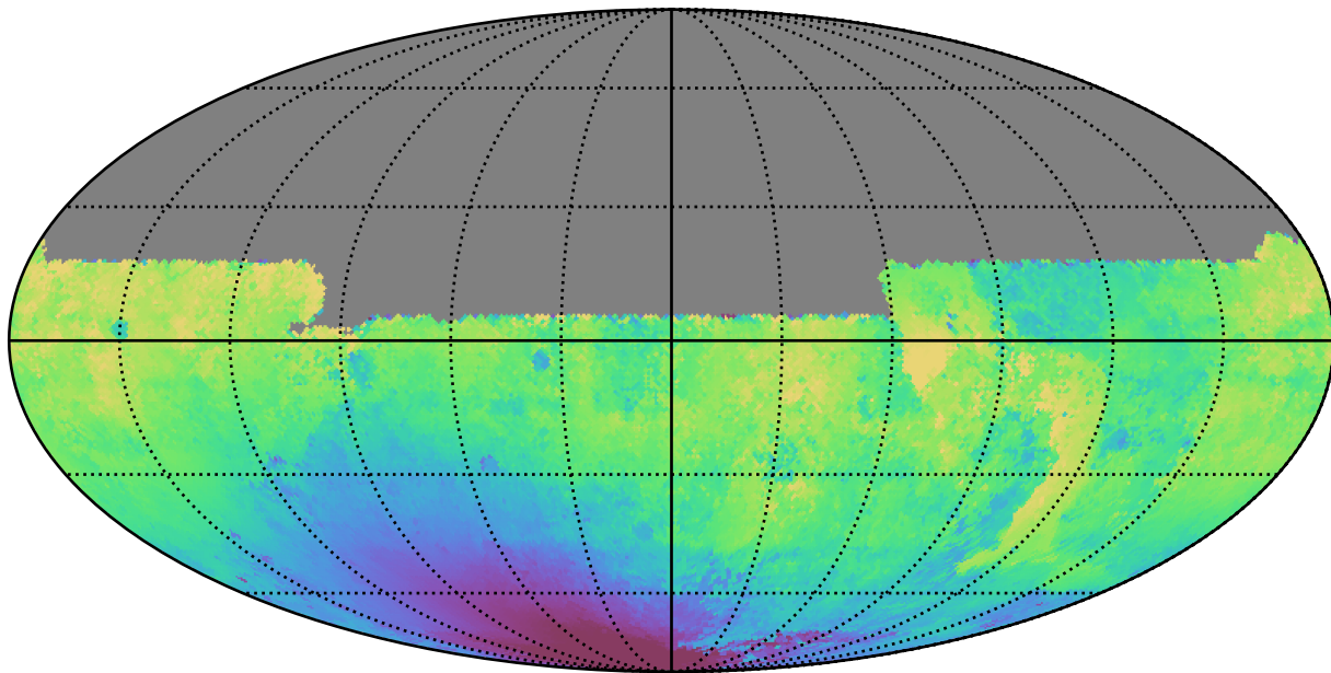
all_long_v3.4_10yrs All sky u band: Median solarElong
