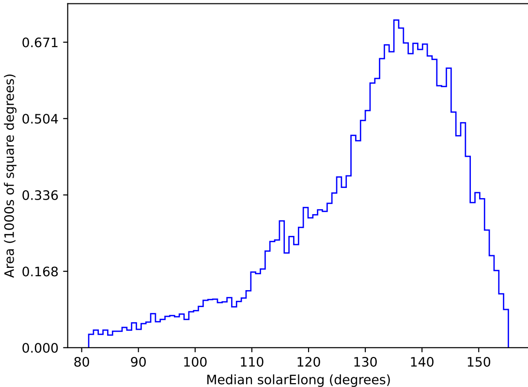
all_long_v3.4_10yrs All sky u band: Median solarElong
