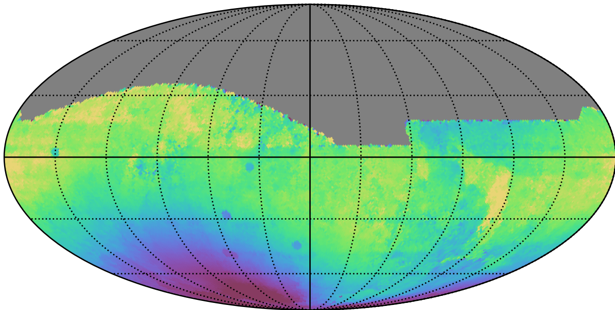
all_long_v3.4_10yrs All sky r band: Median solarElong
