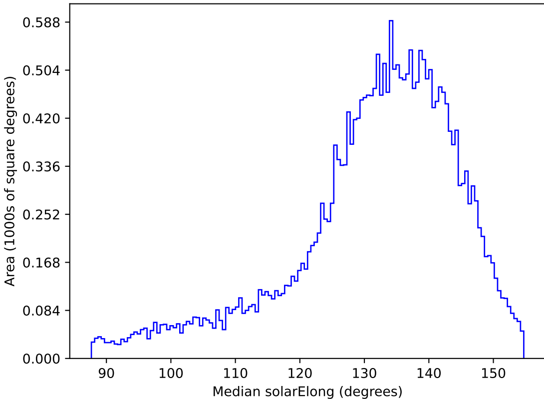
all_long_v3.4_10yrs All sky i band: Median solarElong
