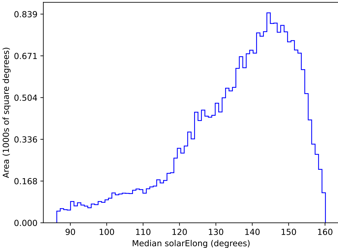
all_long_v3.4_10yrs All sky g band: Median solarElong
