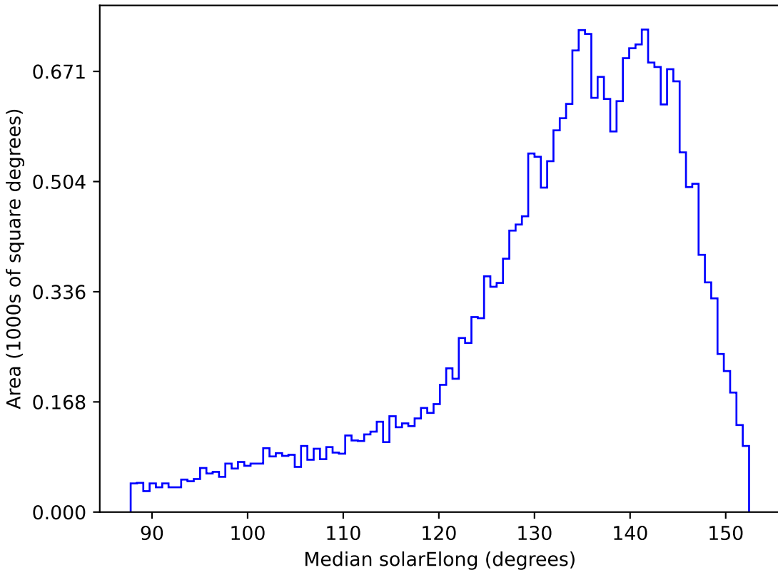
all_long_v3.4_10yrs All sky all bands: Median solarElong
