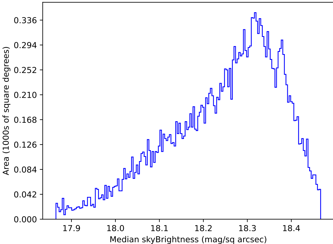
all_long_v3.4_10yrs Yr 1 y band: Median skyBrightness
