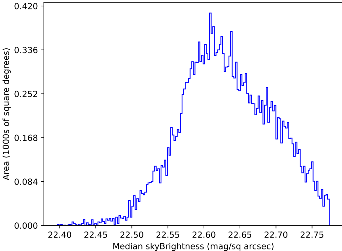
all_long_v3.4_10yrs Yr 1 u band: Median skyBrightness
