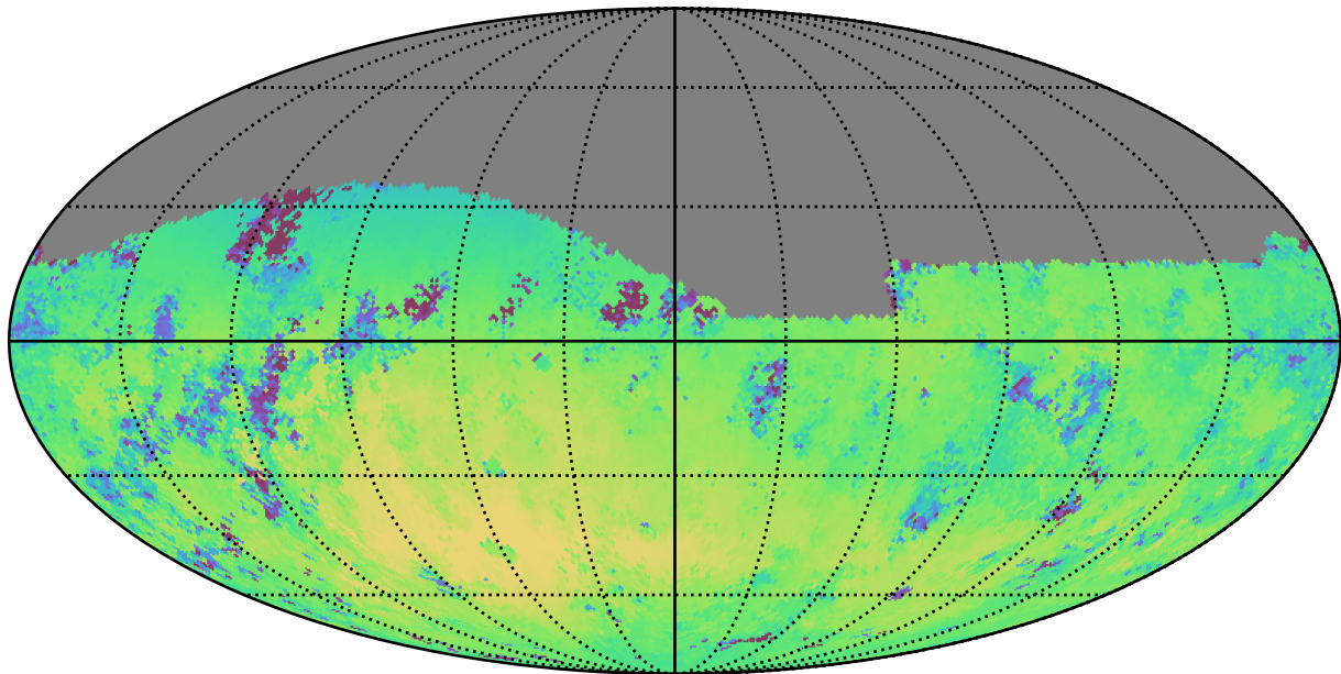
all_long_v3.4_10yrs Yr 1 r band: Median skyBrightness
