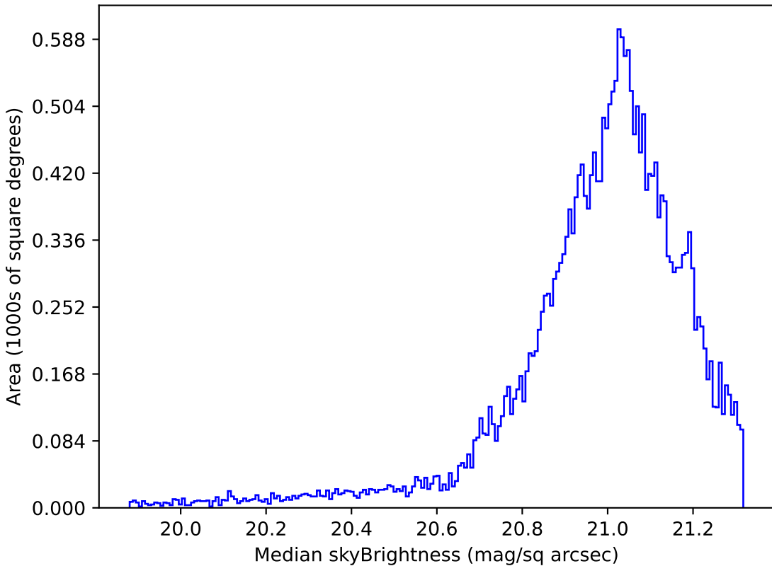
all_long_v3.4_10yrs Yr 1 r band: Median skyBrightness
