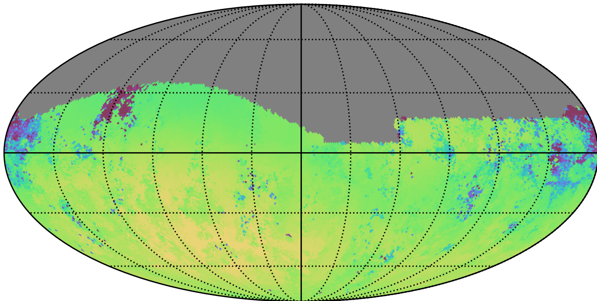
all_long_v3.4_10yrs Yr 1 g band: Median skyBrightness
