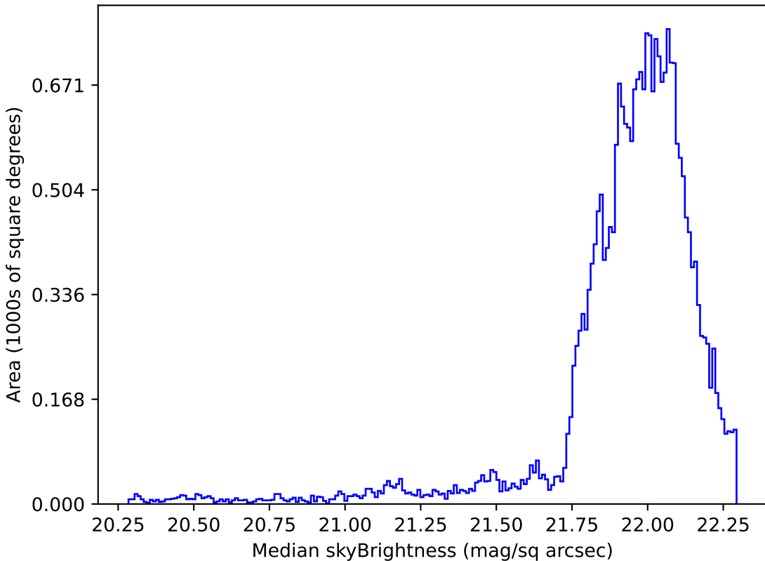
all_long_v3.4_10yrs Yr 1 g band: Median skyBrightness
