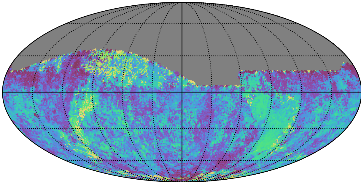
all_long_v3.4_10yrs Yr 1 all bands: Median skyBrightness
