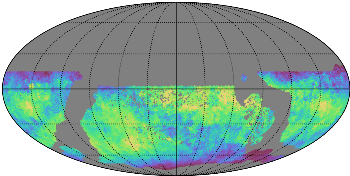
all_long_v3.4_10yrs WFD z band: Median skyBrightness
