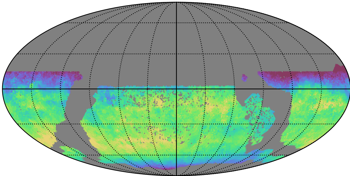
all_long_v3.4_10yrs WFD y band: Median skyBrightness
