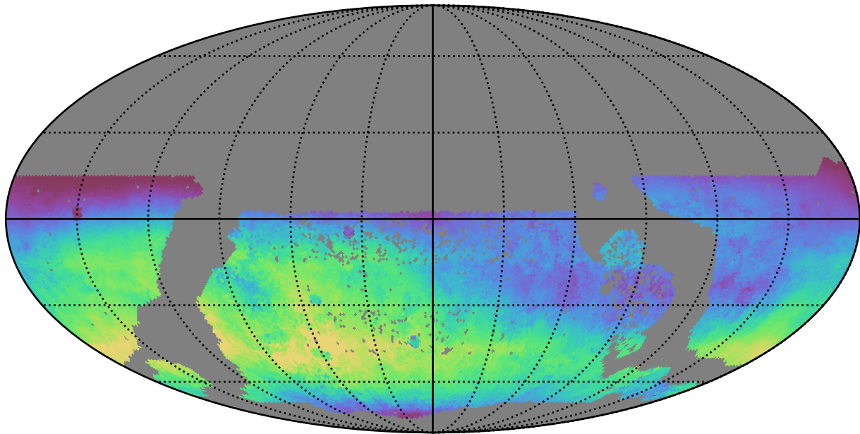
all_long_v3.4_10yrs WFD u band: Median skyBrightness
