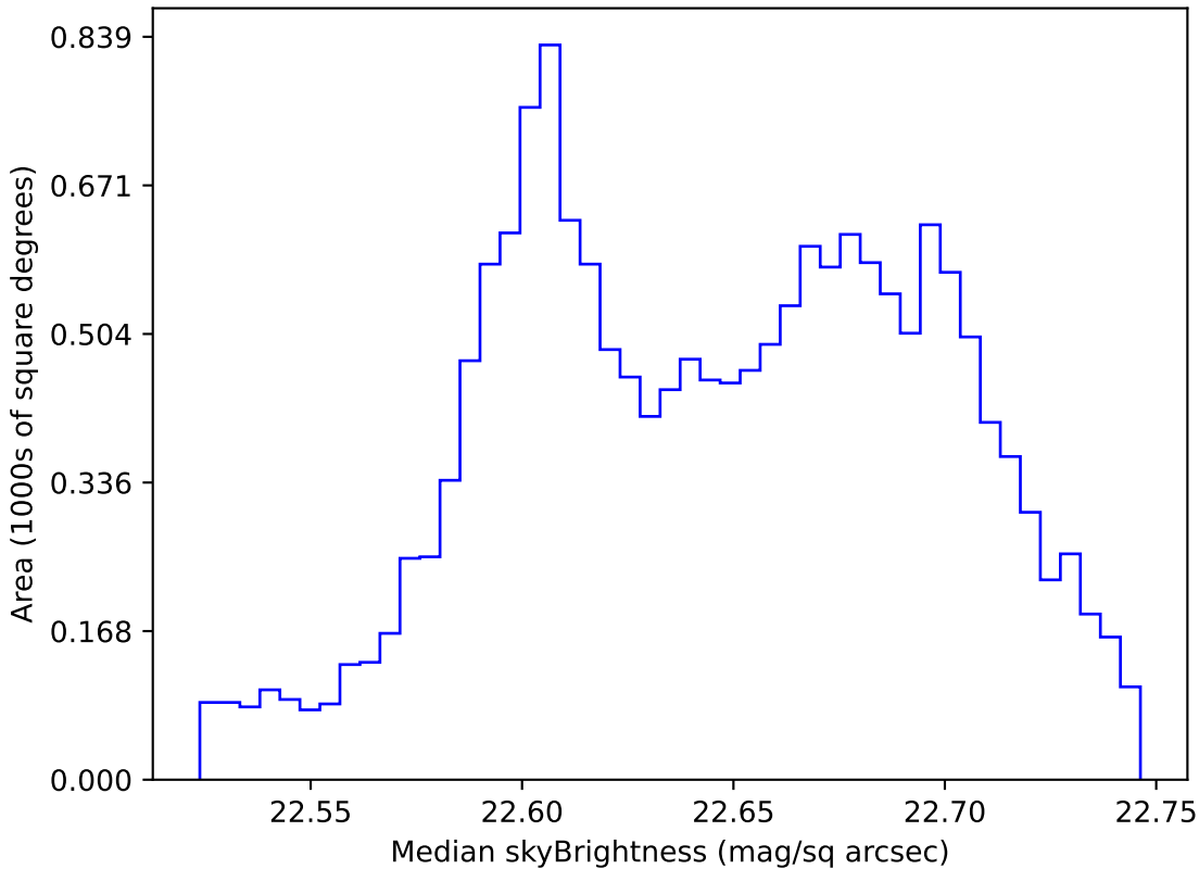
all_long_v3.4_10yrs WFD u band: Median skyBrightness
