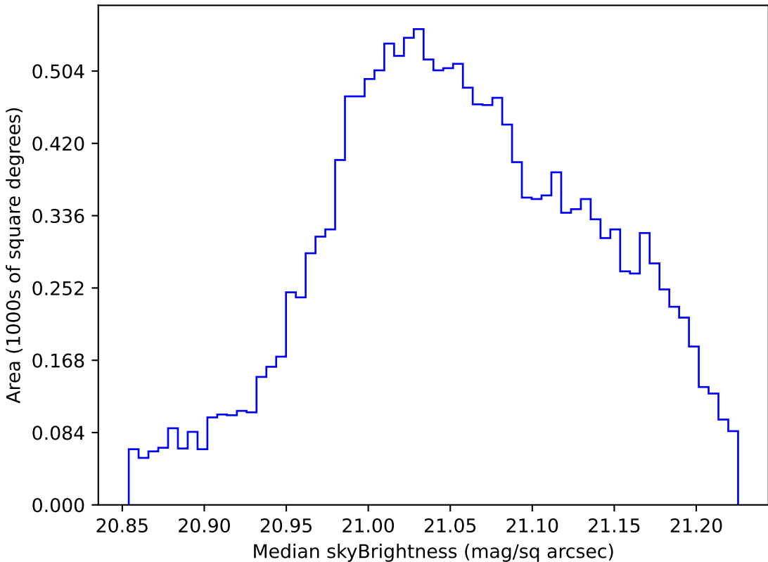
all_long_v3.4_10yrs WFD r band: Median skyBrightness
