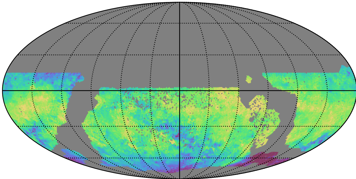
all_long_v3.4_10yrs WFD i band: Median skyBrightness
