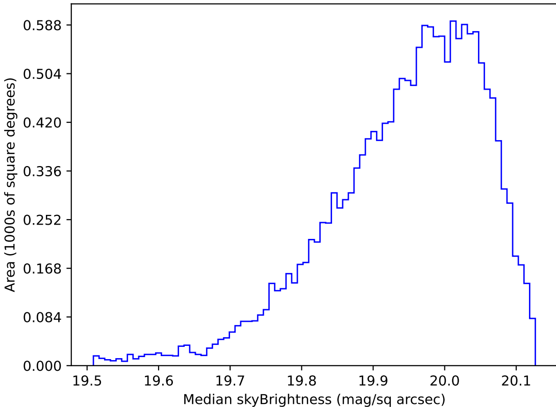
all_long_v3.4_10yrs WFD i band: Median skyBrightness
