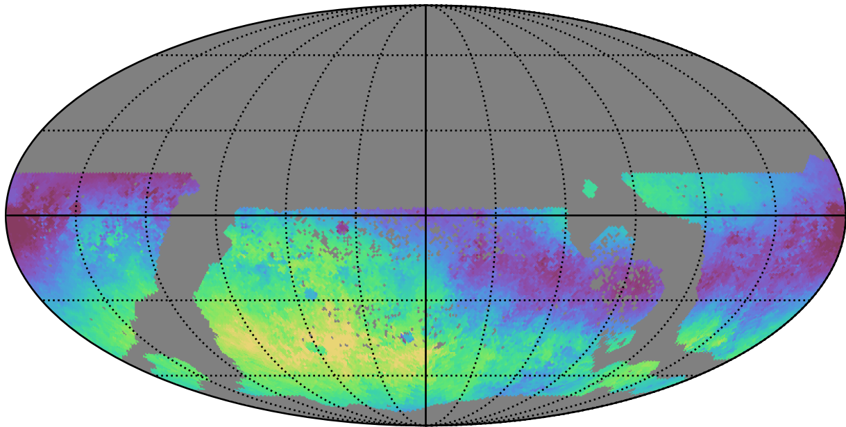
all_long_v3.4_10yrs WFD g band: Median skyBrightness
