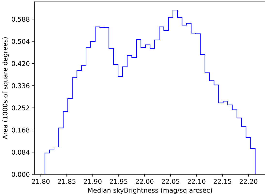
all_long_v3.4_10yrs WFD g band: Median skyBrightness
