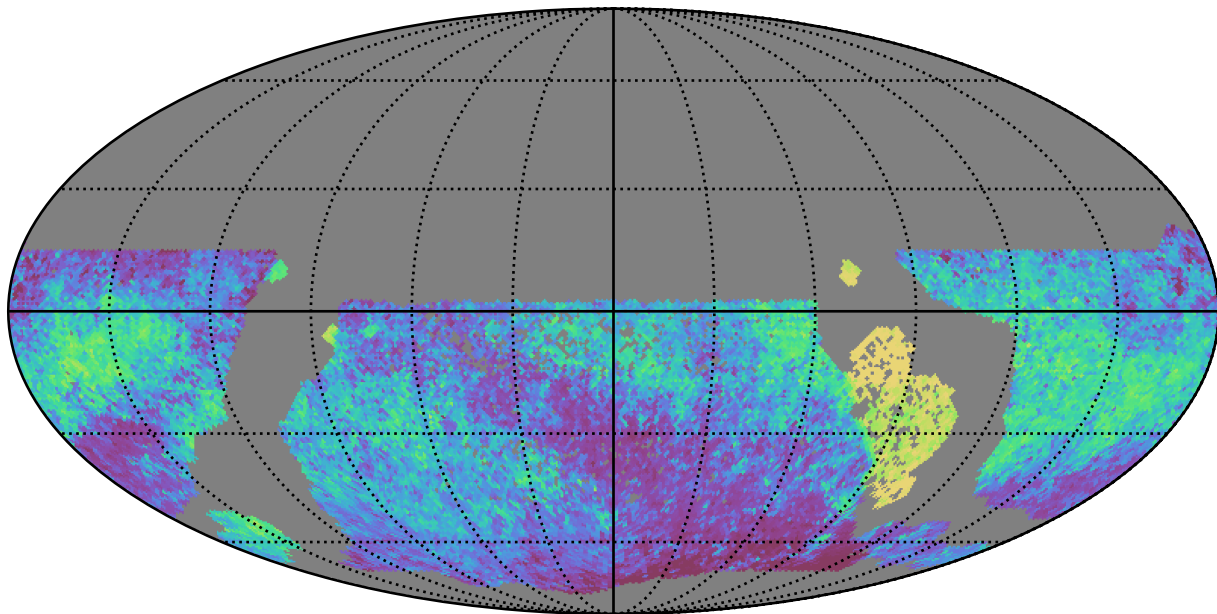
all_long_v3.4_10yrs WFD all bands: Median skyBrightness
