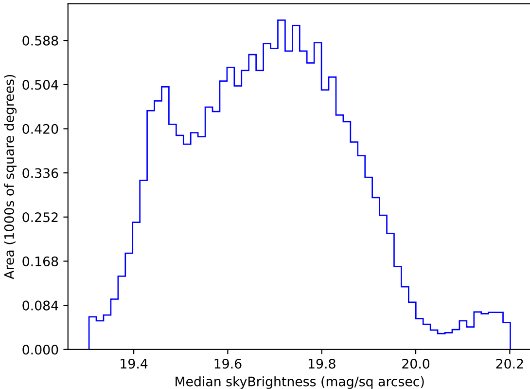
all_long_v3.4_10yrs WFD all bands: Median skyBrightness
