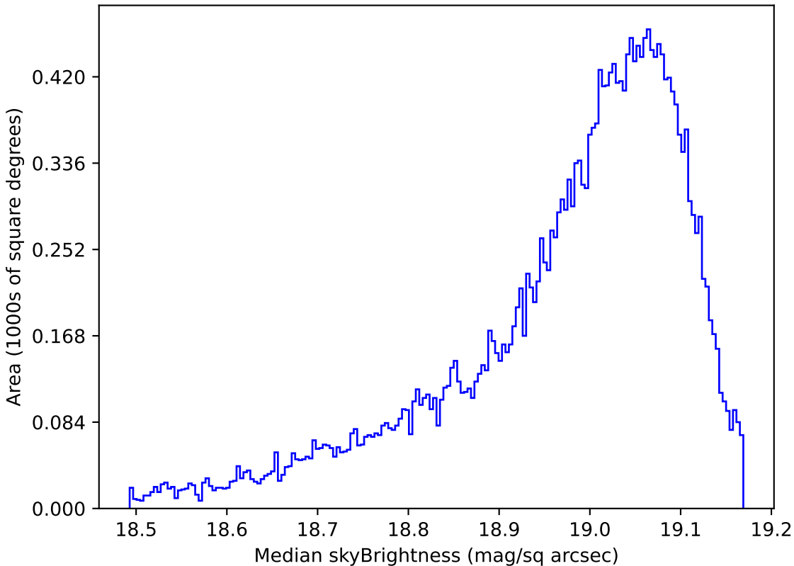
all_long_v3.4_10yrs All sky z band: Median skyBrightness
