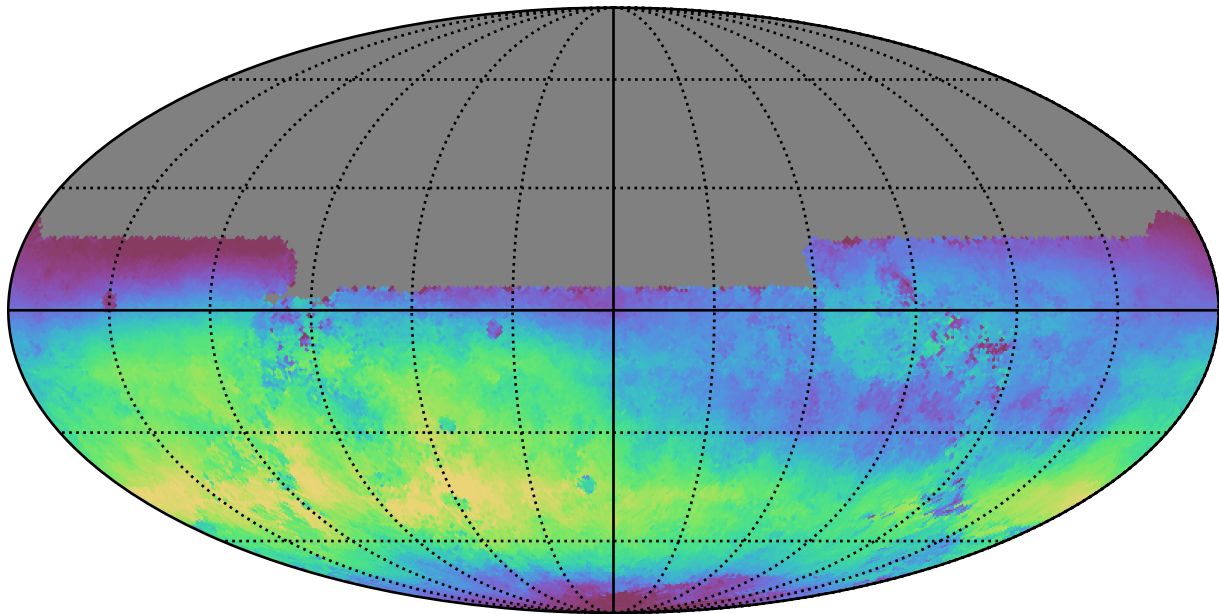
all_long_v3.4_10yrs All sky u band: Median skyBrightness
