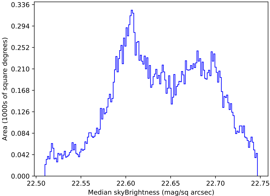
all_long_v3.4_10yrs All sky u band: Median skyBrightness
